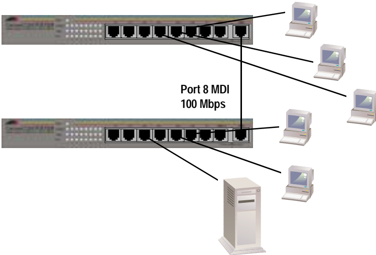
Figure 5 Cascading Switches
