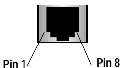
Figure 7 RJ45 Connector
